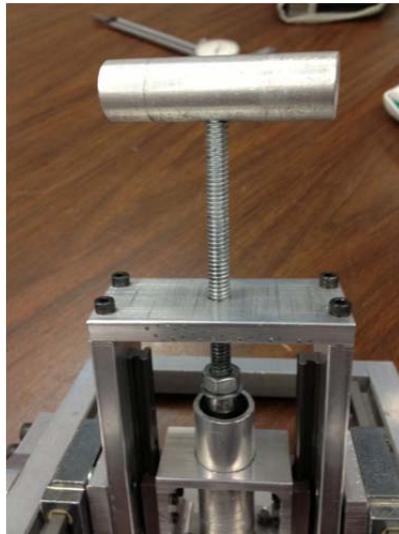
Figure 10: Handle Assembly
